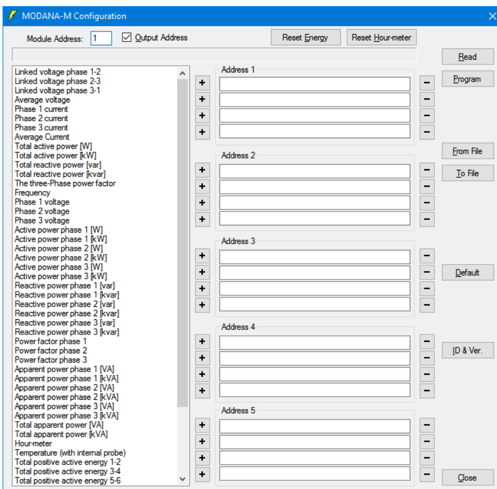
Figure 1: ModANA-M configuration panel
